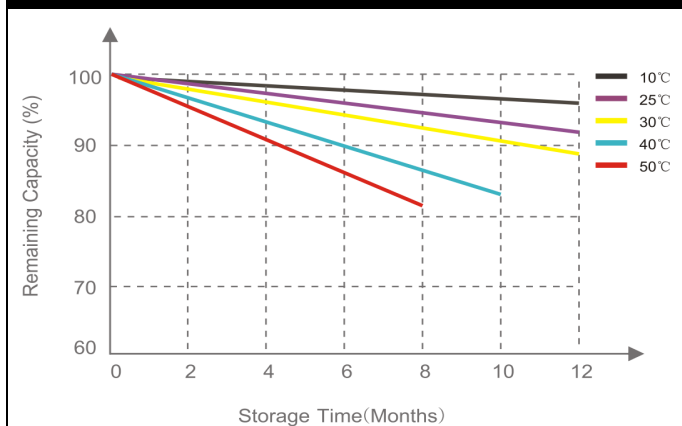
Self Discharge Curve at Different Temperatures
